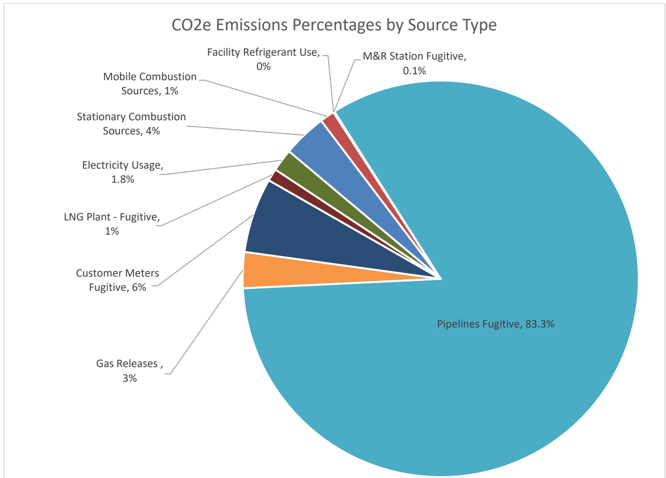
Figure 1-1. CY2016 PGW Greenhouse Gas Emissions by Source Category
