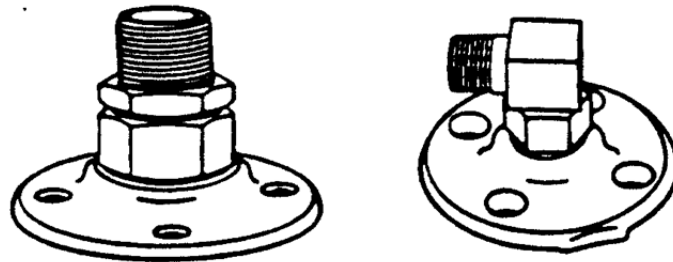
TERMINATION FITTING
